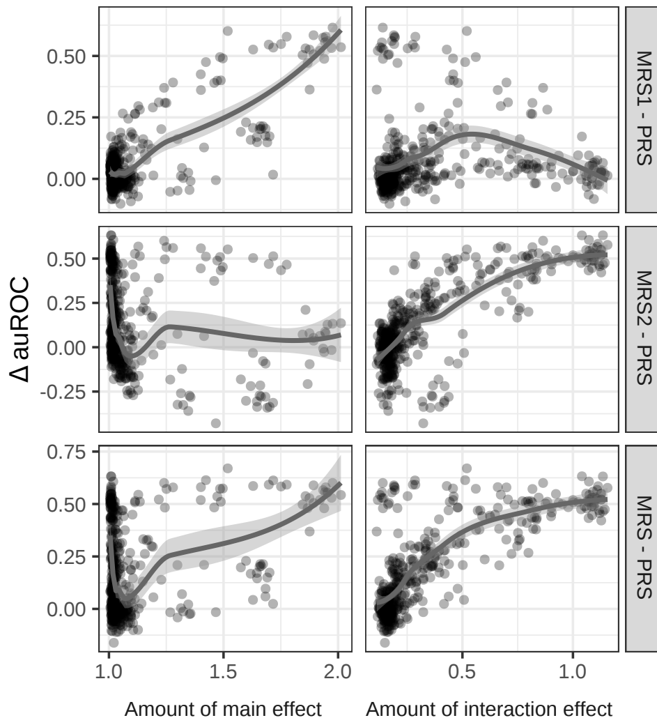
Figure 2: Combining 1-way (MRS1) and 2-way (MRS2) risk scores, MRS shows increasing outperformance to standard PRS as dataset contains more main and interaction effects.
